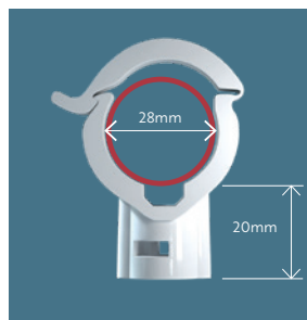
28mm ecoclip weight - 17g
